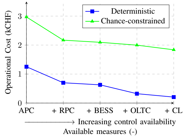
Fig. 10. Operational costs for different sets of active measures. APC = Active Power Curtailment, RPC = Reactive Power Control, BESS = Battery Energy Storage System, OLTC = On Load Tap Changing transformer, CL = Controllable Load
