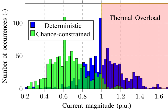
Fig. 12. Histogram of the current magnitudes at 14:00 at Cable 2 – 3, evaluated based on Monte Carlo samples for both the deterministic (blue) and chance-constrained (green) solutions.
