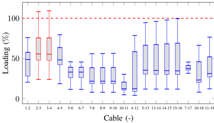
Fig. 9. Boxplots for the daily thermal loading of the cables. Each boxplot shows the minimum, the first quartile, the median, the third quartile, and the maximum value over the time considered.
